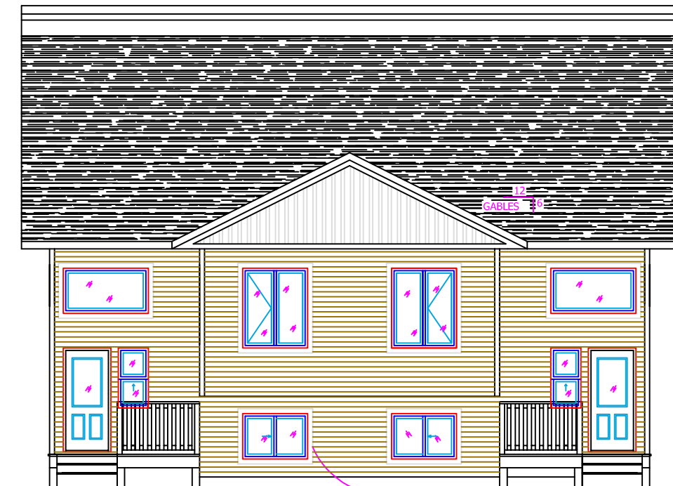
Rear Unit Elevation
