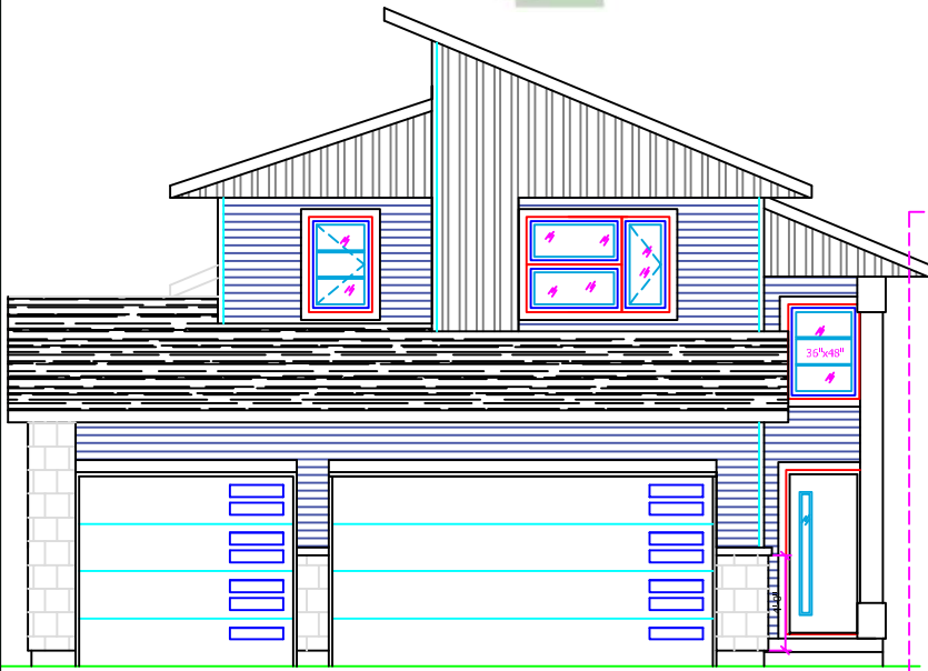
Front Elevation 122 Mitchell Cres
