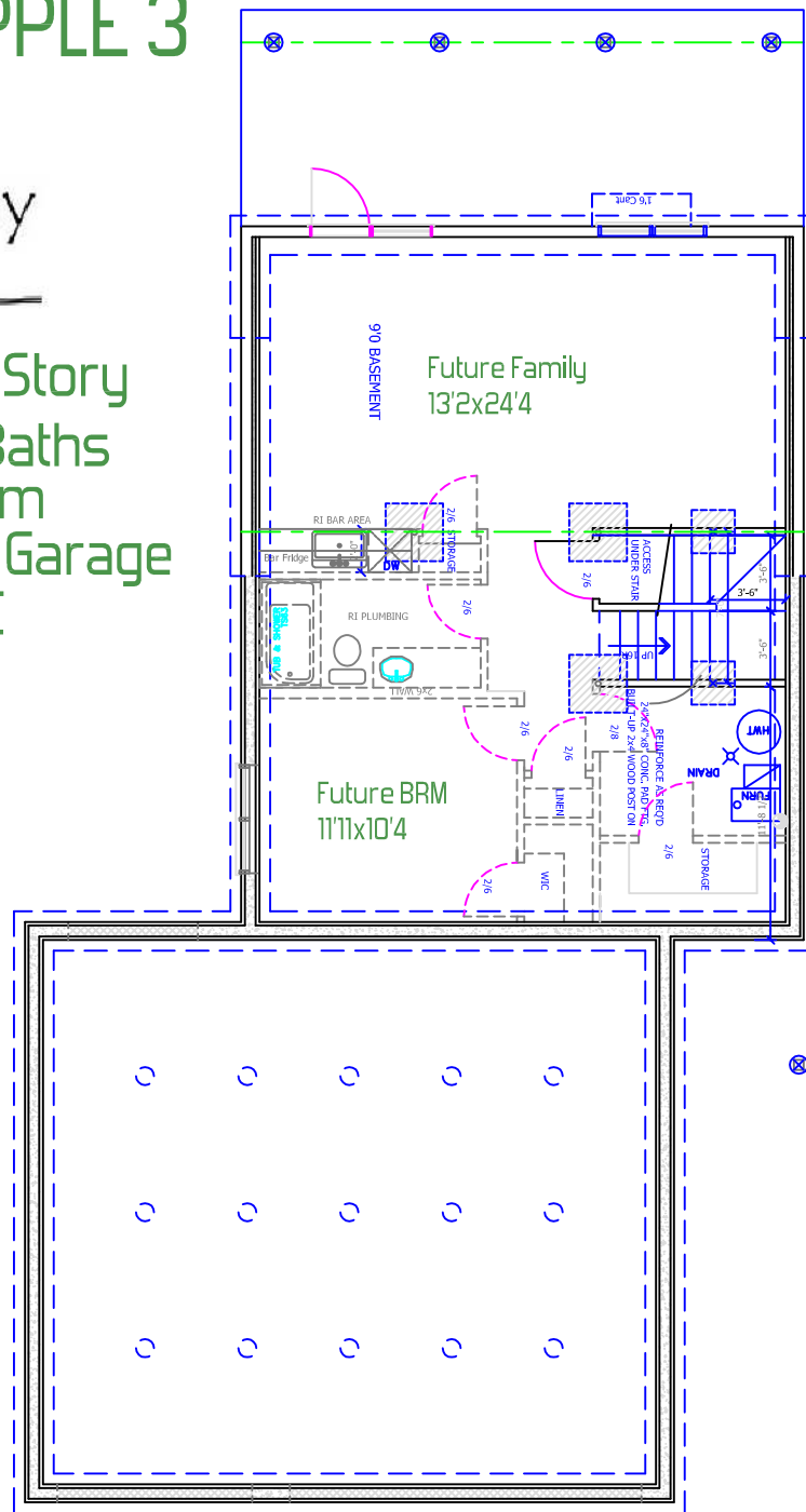
Lower Floor
