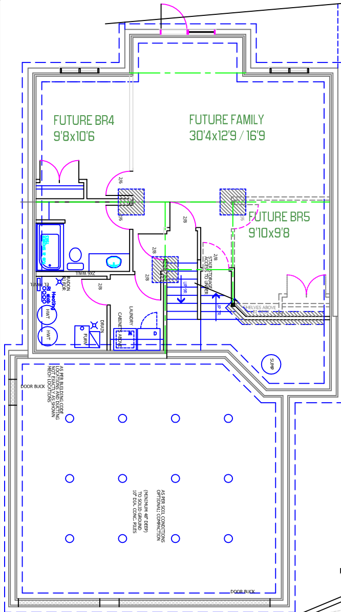
Foundation Plan
