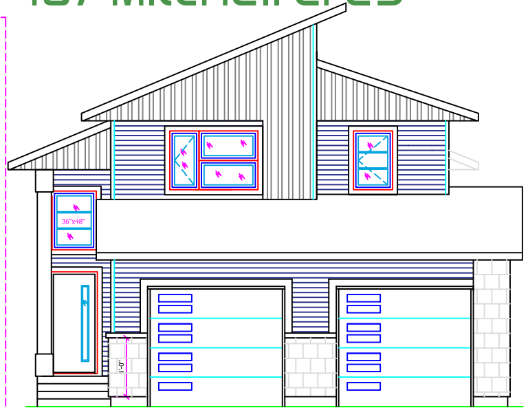
Front Elevation
