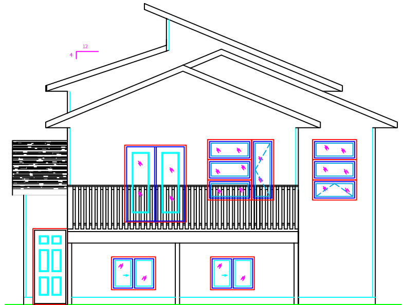
Rear Elevation
