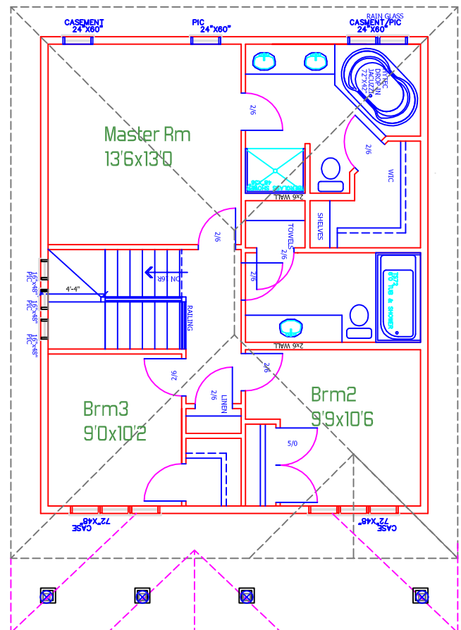
UPPER FLOOR PLAN 769 Sqft
